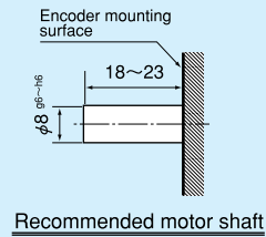
Recommended motor shaft
