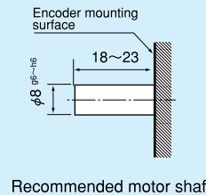
Recommended motor shaft
