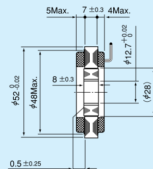
Mounting method of a stator and a rotor in the axial direction
