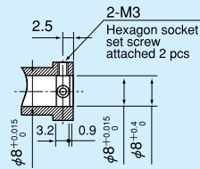
Shaft details
