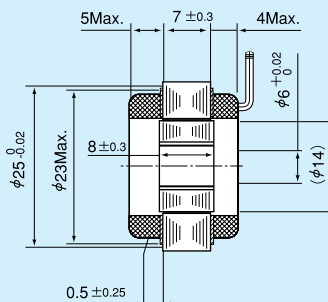
Mounting method of a stator and a rotor in the axial direction
