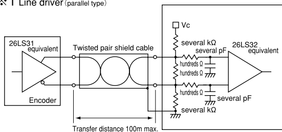
※1 Line driver (parallel type)
