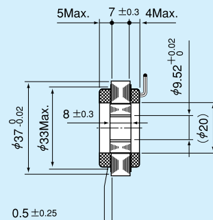
Mounting method of a stator and a rotor in the axial direction
