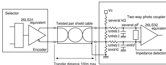
※2 Line driver (wire-saving type)
