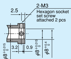
Shaft details
