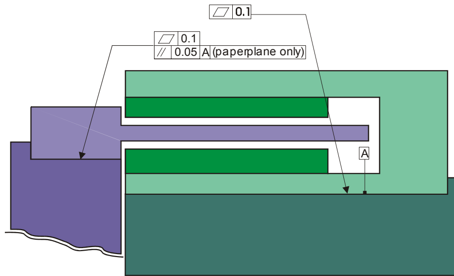
Figure 7: Flatness and parallelism of mounting surfaces, schematically
