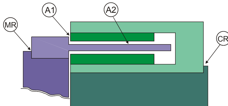
Figure 8: Air gaps and axial references, schematically
