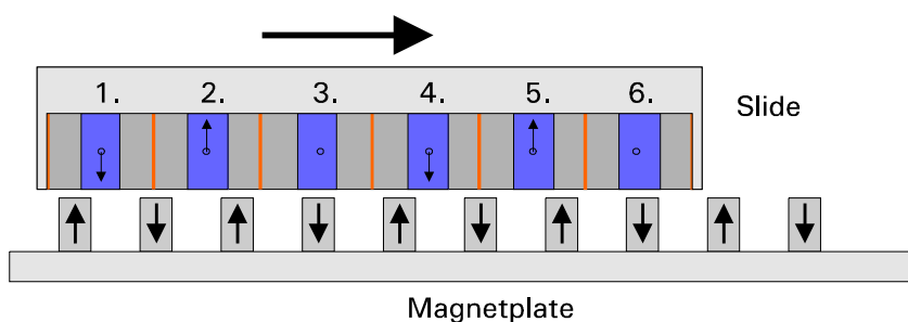
Figure 11: Positioning and phasing for a 3 phase linear motor
