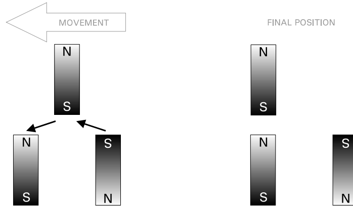
Figure 6: Moving principle 1
