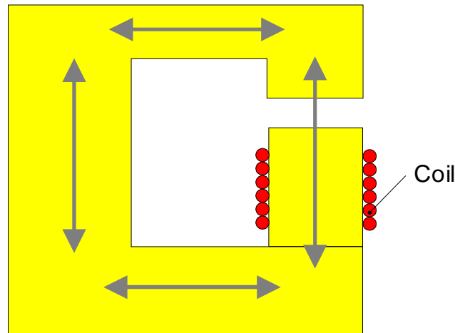
Figure 5: Elementary magnetic circuit
