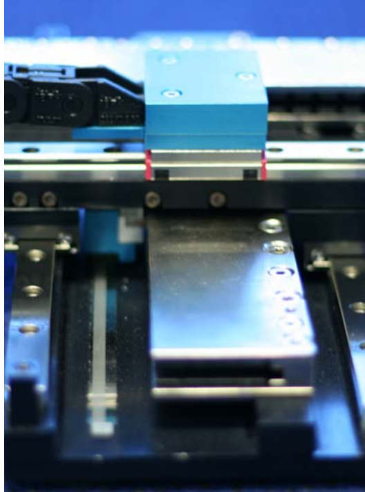
Figure 24: Ironless linear motor system (UC3)
