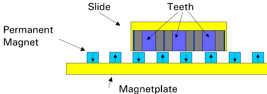
Figure 8: Linear motor, schematic cross section
