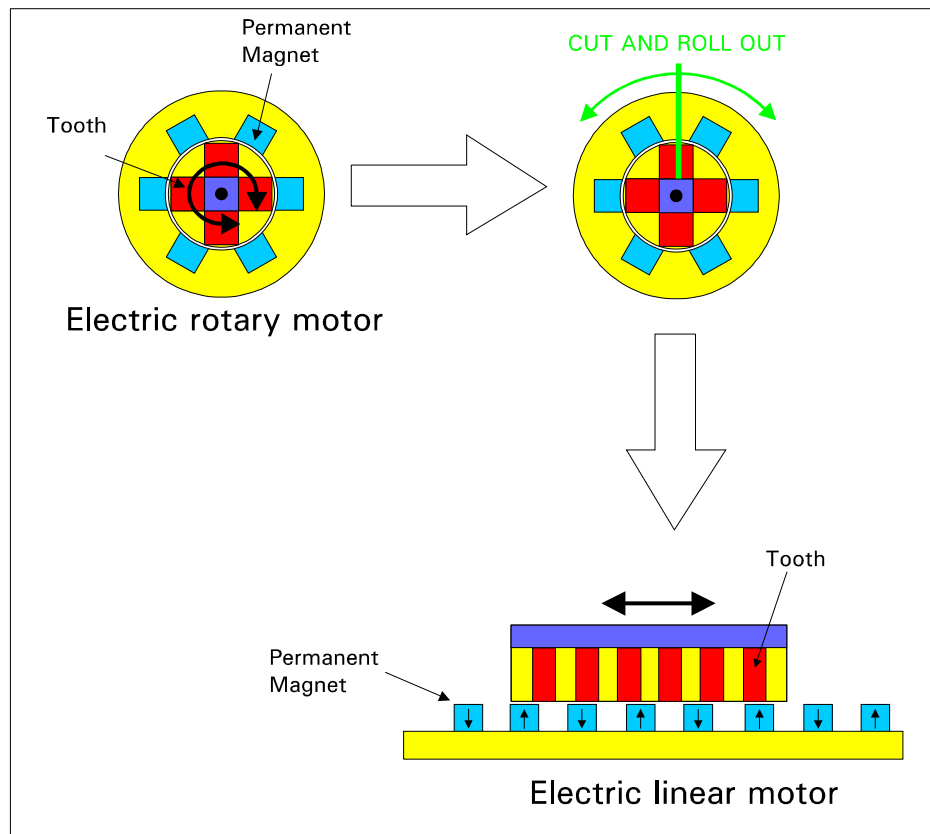
Figure 18: A rotary motor opened up and laid out flat
