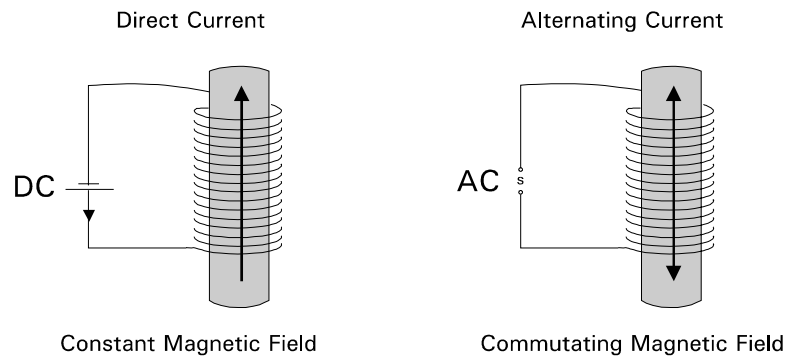
Figure 3: Electromagnetic exciting of a constant and a commutating magnetic field
