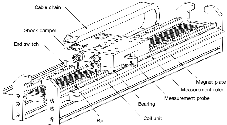
Figure 20: Ironcore linear motor system, example
