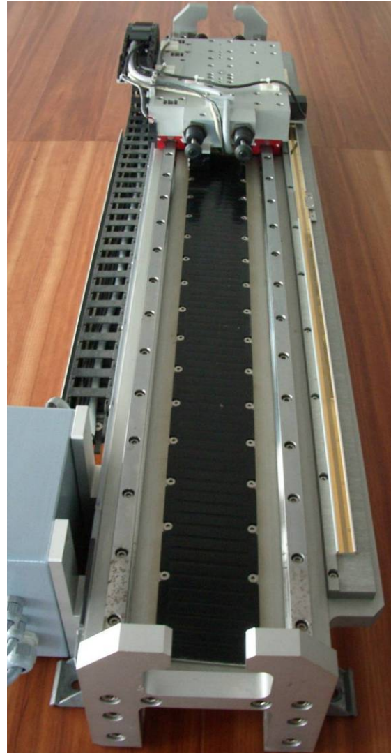
Figure 21: Ironcore linear motor system
