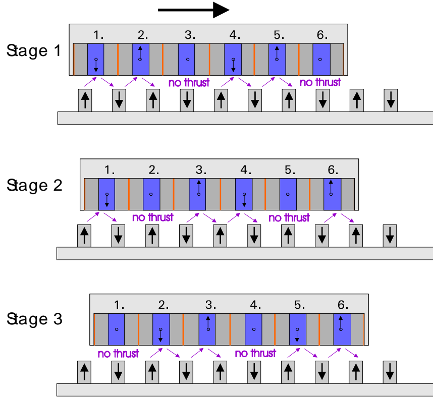
Figure 12: Stages of the 3 phase linear motor's motion
