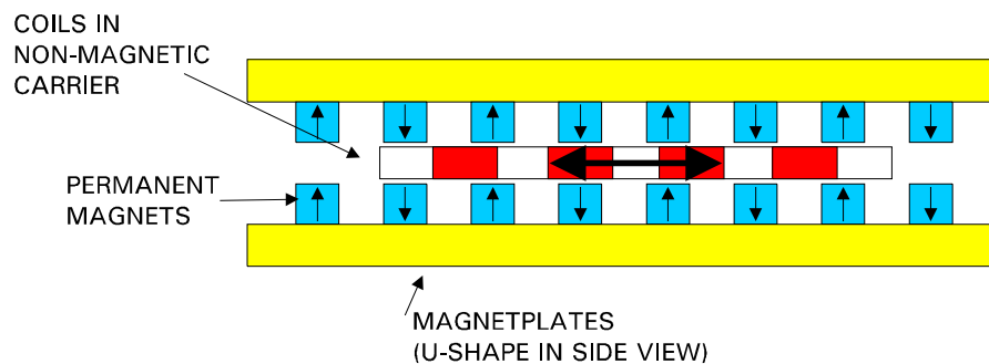
Figure 17: Ironless linear motor, schematic cross section
