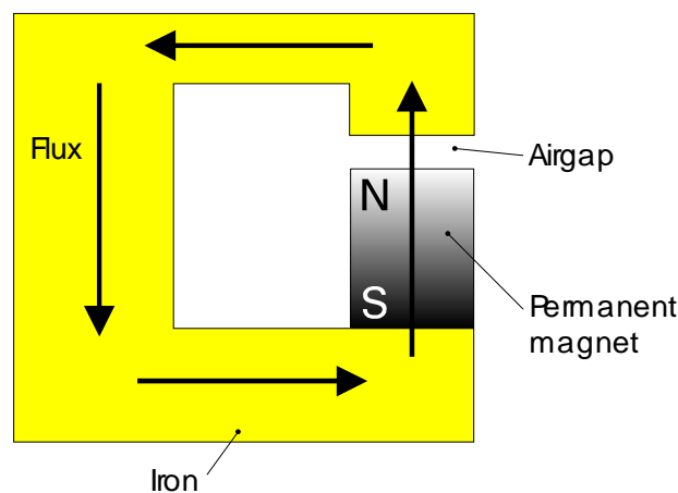
Figure 4: Elementary magnetic circuit
