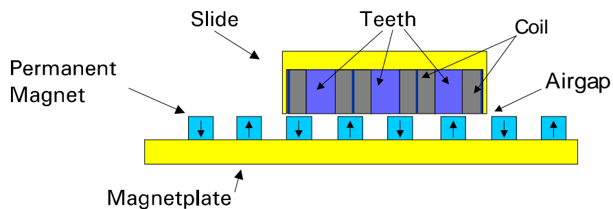
Figure 15: Ironcore linear motor, schematic cross section
