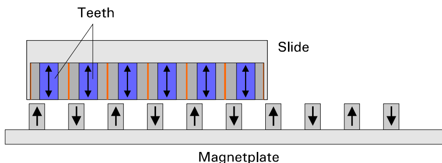
Figure 10: Erroneous positioning and phasing
