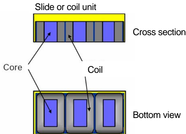
Figure 9: Coil unit with three coils, schematic
