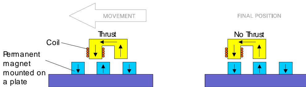
Figure 7: Moving principle 2
